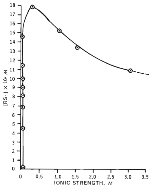
Figure 3 —Concentration of thiol free radicals observed upon oxidation of 0.02 M cysteine hydrochloride by 0.005 M CeK_2(NO_3)_6 as a function of ionic strength.
