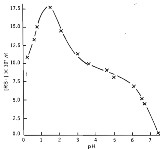
Figure 1 —pH dependency of thiol free radicals generated upon oxidation of 0.02 M cysteine hydrochloride with 0.005 M \text{CeK}_2(\text{NO}_3)_6 .
