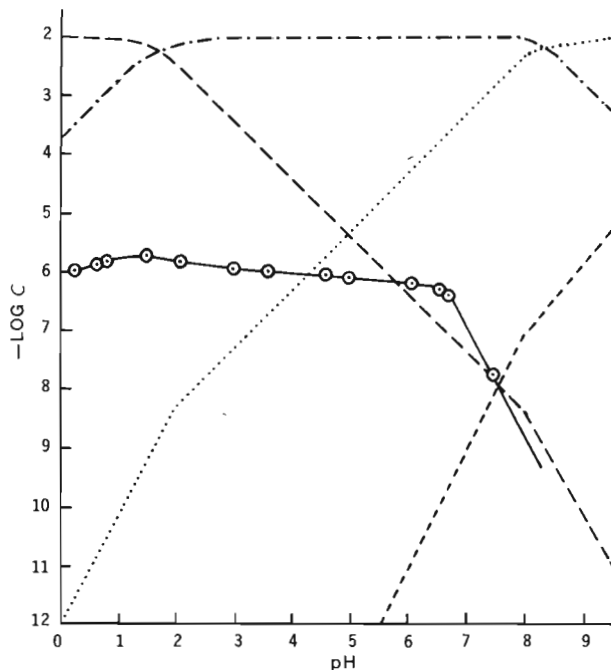
Figure 2 —Relation of the thiyl free radical concentration observed during ceric-ion oxidation of cysteine hydrochloride to the concentration of the different ionic forms of cysteine as a function of pH. Key: C, concentration of free radical or ionic species: —, RS\cdot ; ---, \text{HSCH}_2\text{CH}(\text{NH}_3^+)\text{COOH} ; - · - · - ·, \text{HSCH}_2\text{CH}(\text{NH}_3^+)\text{COO}^- ; · · · · ·, -\text{SCH}_2\text{CH}(\text{NH}_3^+)\text{COO}^- ; and - - - - -, -\text{SCH}_2\text{CH}(\text{NH}_2)\text{COO}^- .
